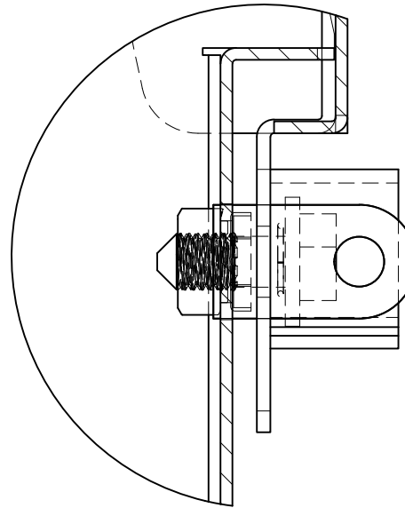
DETAIL I SCALE 1:1.5
